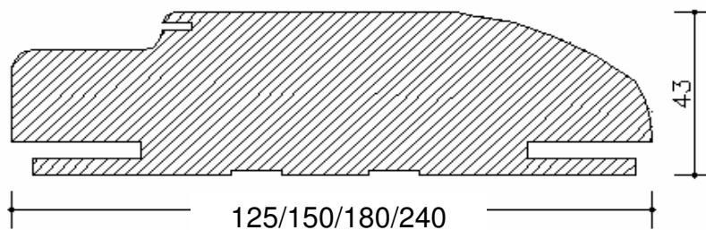
CURVED FRAME
