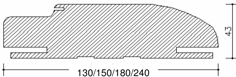
CURVED FRAME
